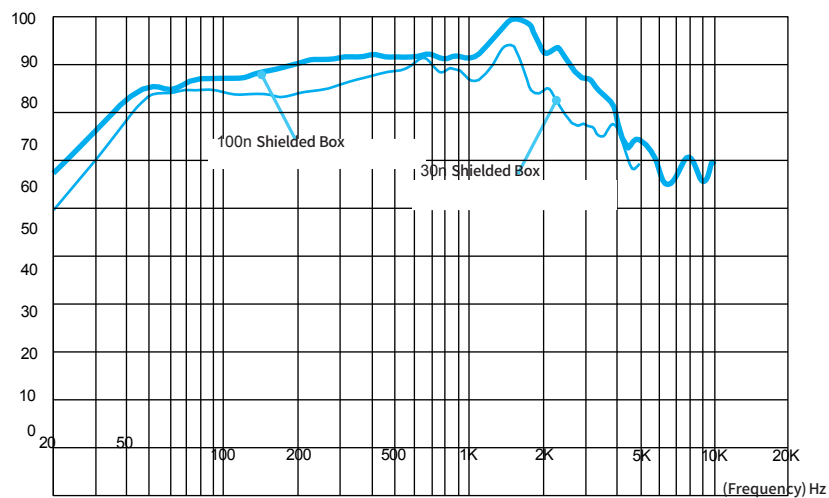
Frequency Response Chart Sound Pressure Output (Anechoic Chamber 1m.1W)
